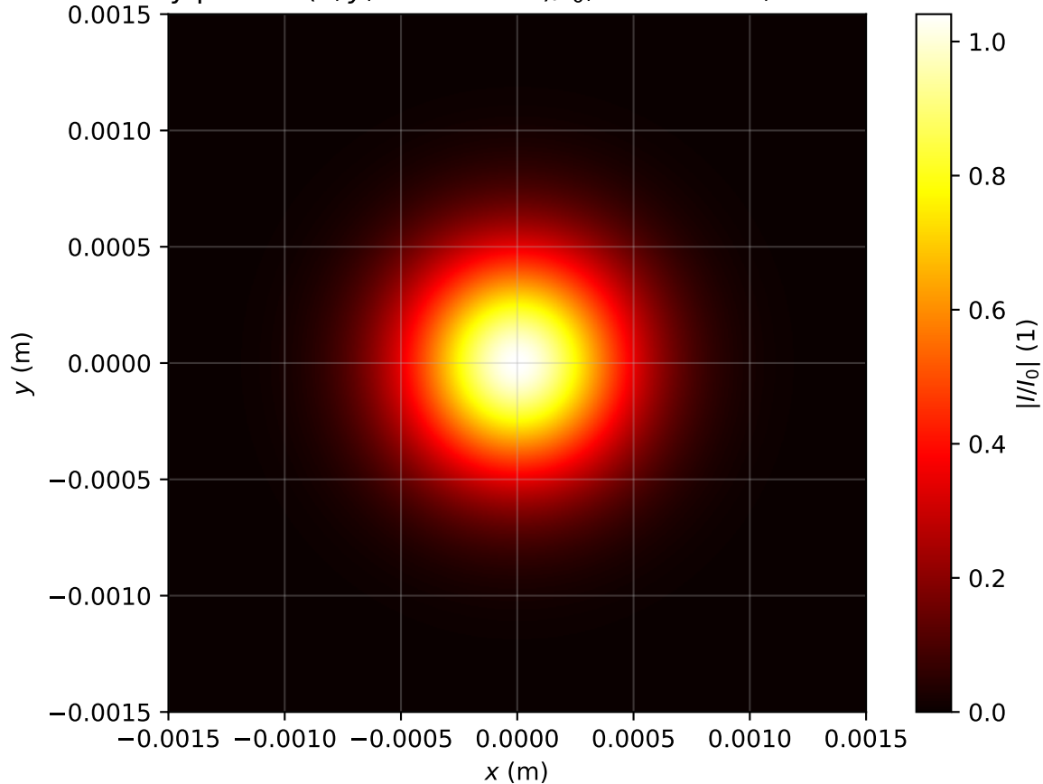
Intensity profile I(x, y, z = 0.478m)/I_0 , P_{in}=0.5P_{cr} , artificial time
